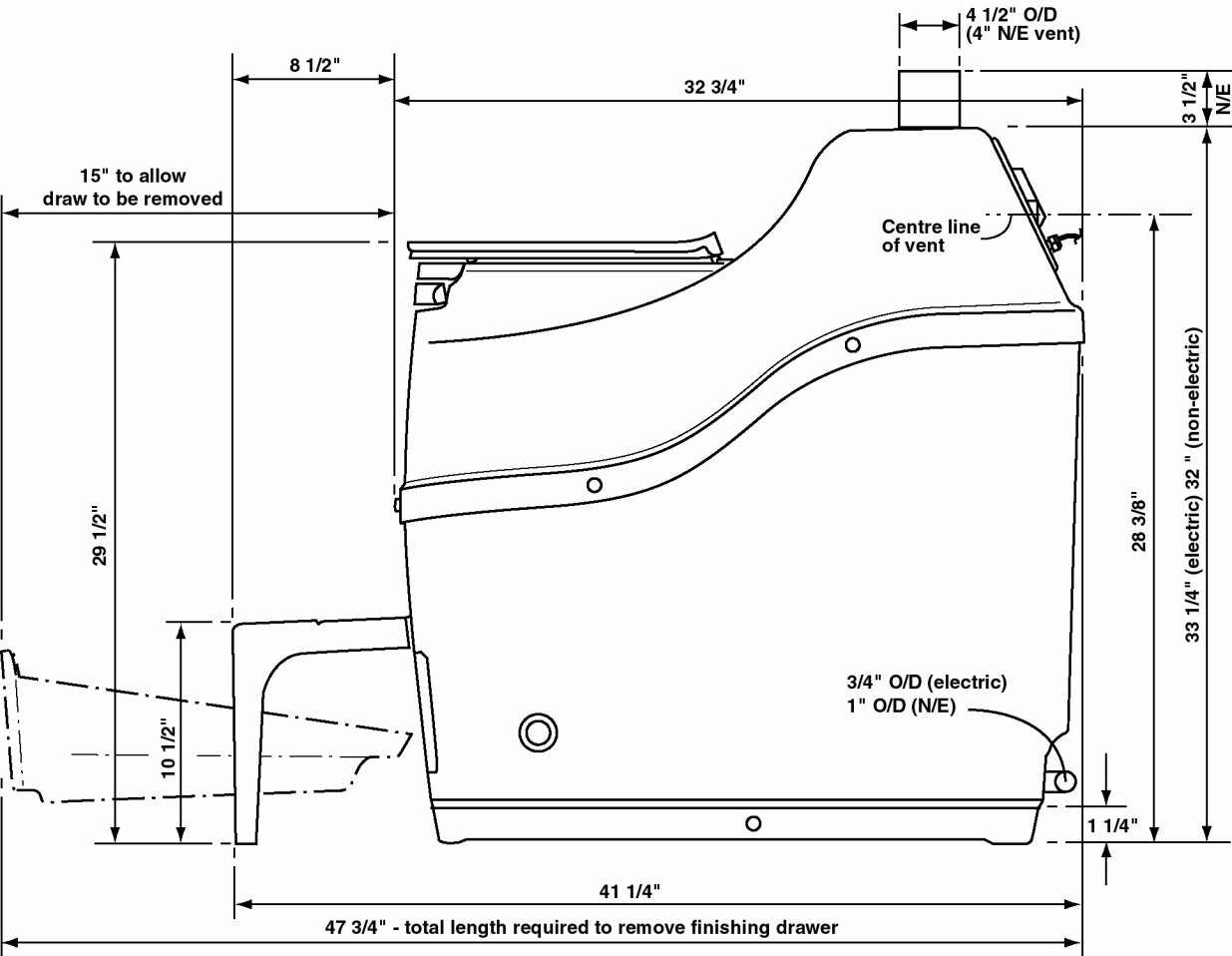
PLAN ELEVATION
