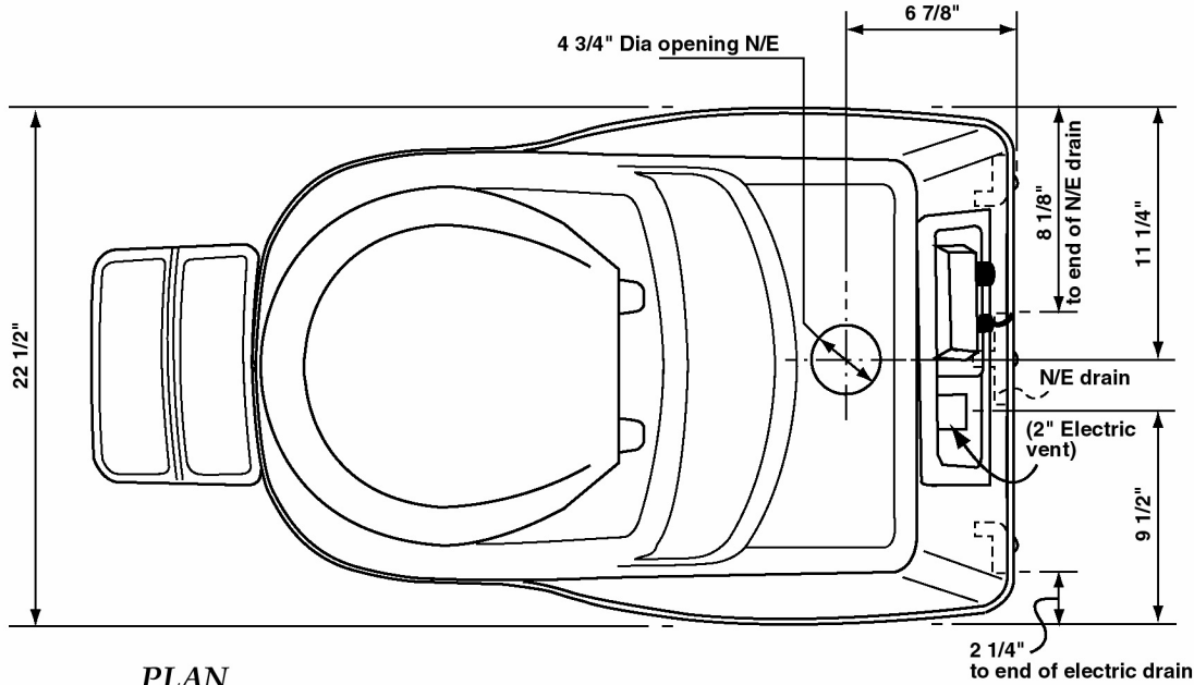
PLAN ELEVATION
